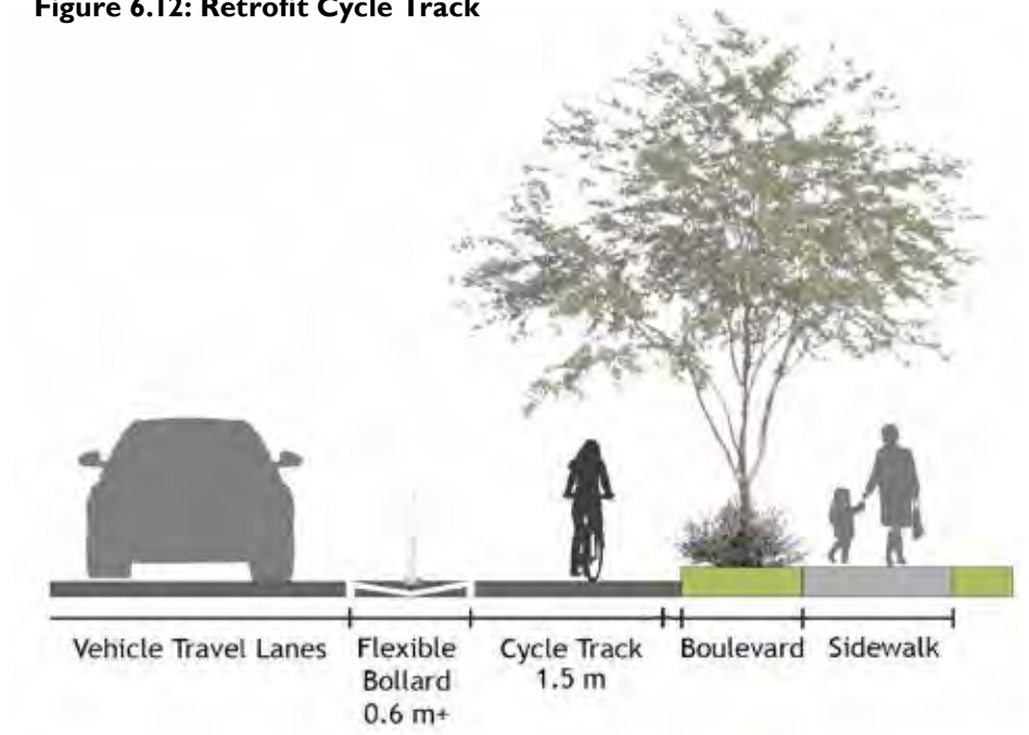
Figure 6.12: Retrofit Cycle Track
