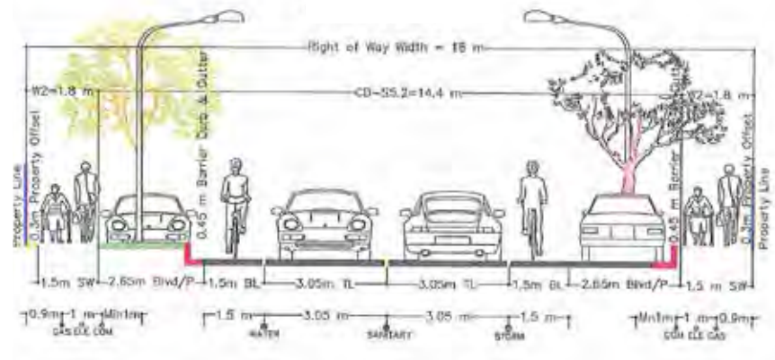
Figure 7.2: Proposed Section for Local Through Streets
