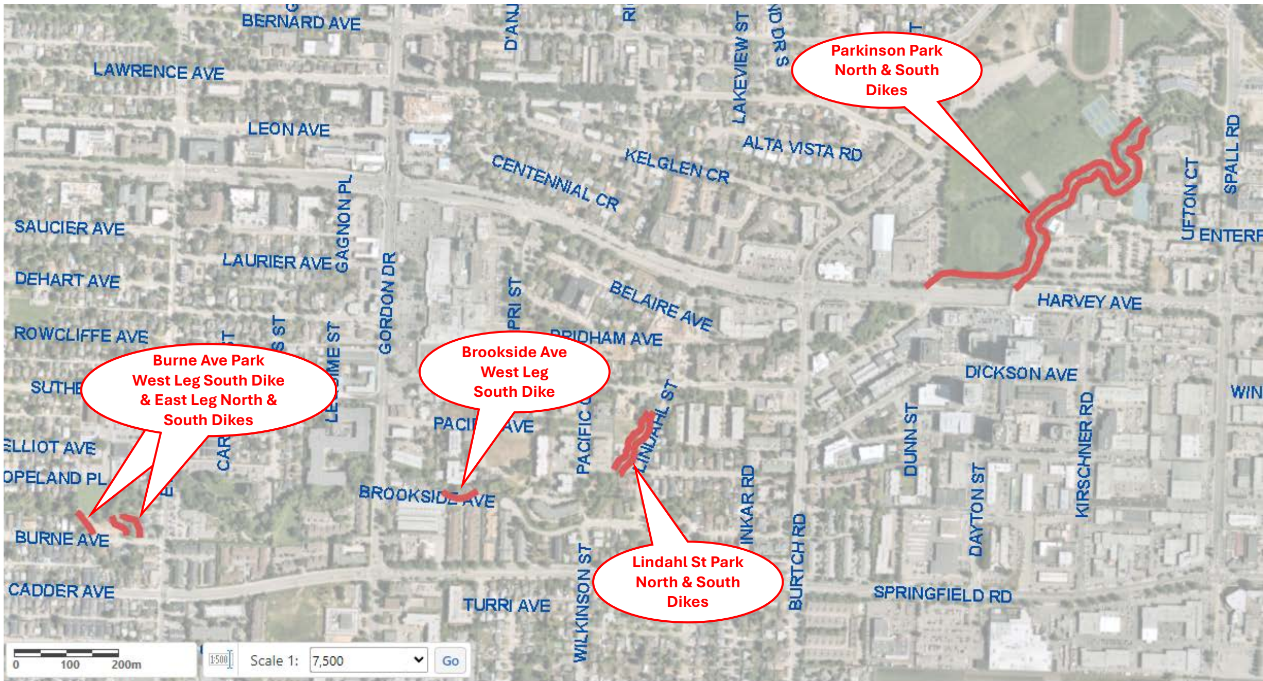
Figure 1. Lower Mill Creek Planned Diking
