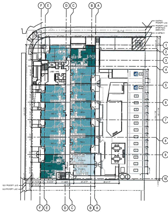
2 FLOOR PLAN - LEVEL 1 SCALE: 1/8" = 1'-0"
