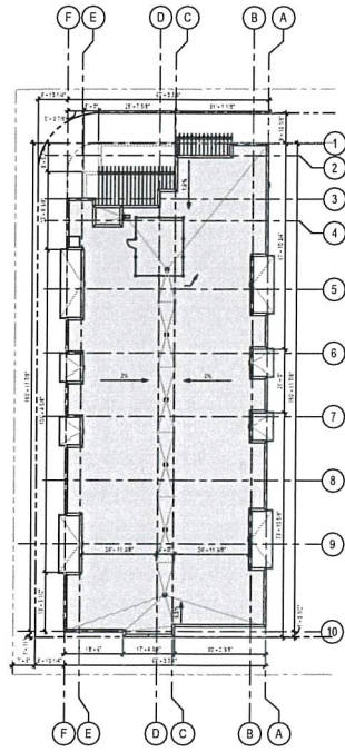
3 ROOF PLAN SCALE: 1/8" = 1'-0"
