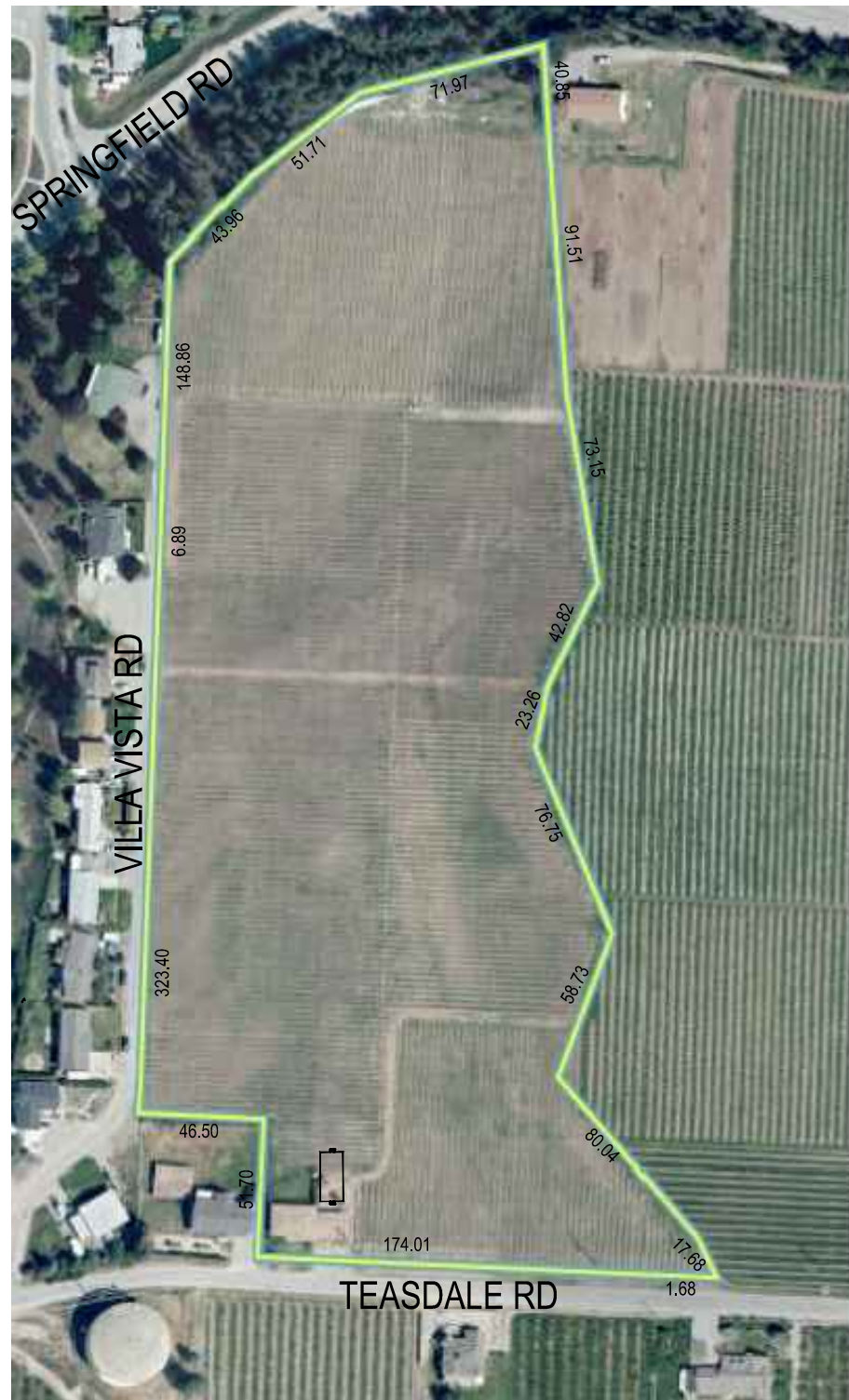
1 SITE PLAN
