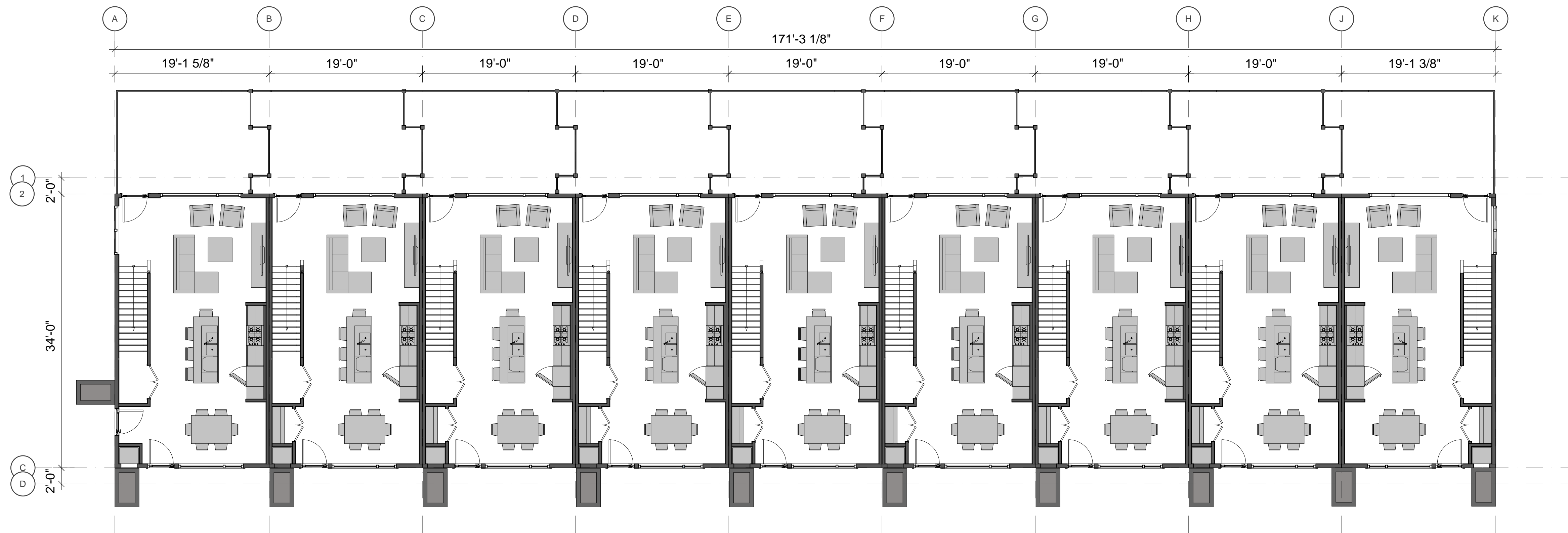
MAIN FLOOR PLAN
