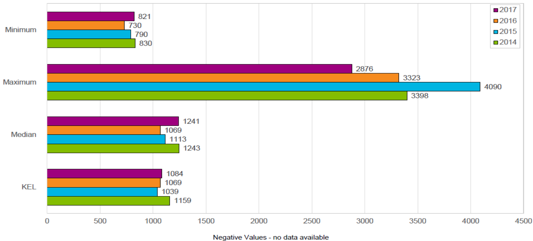
Energy Consumed (kWh) / ML Treated Tertiary WWTPs
