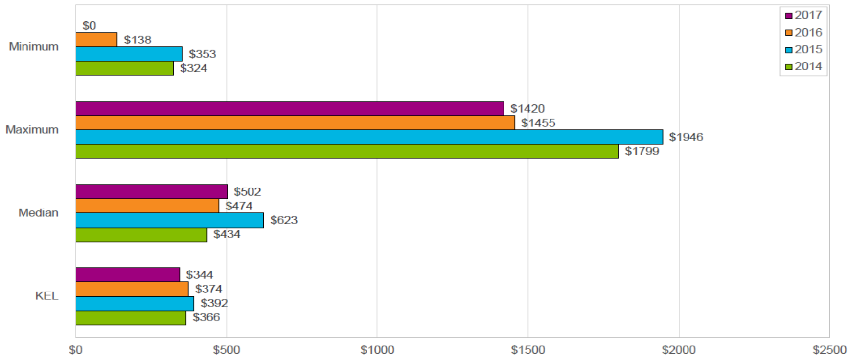
O&M Cost / ML Treated Tertiary WWTPs
