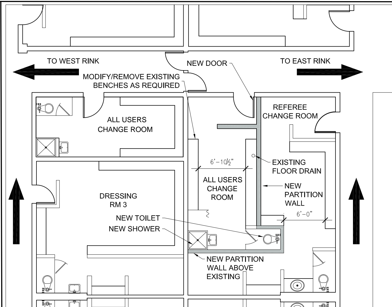
3 PROPOSED RENOVATIONS N.T.S.
