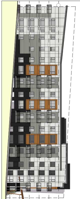
1 WEST ELEVATION
